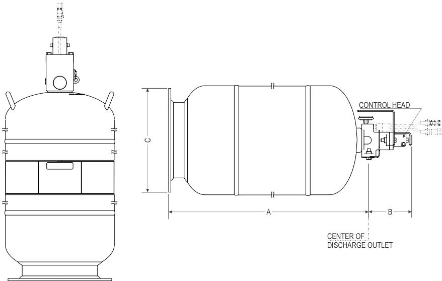
Sentinel LS Cylinders Dimensions [inches]
